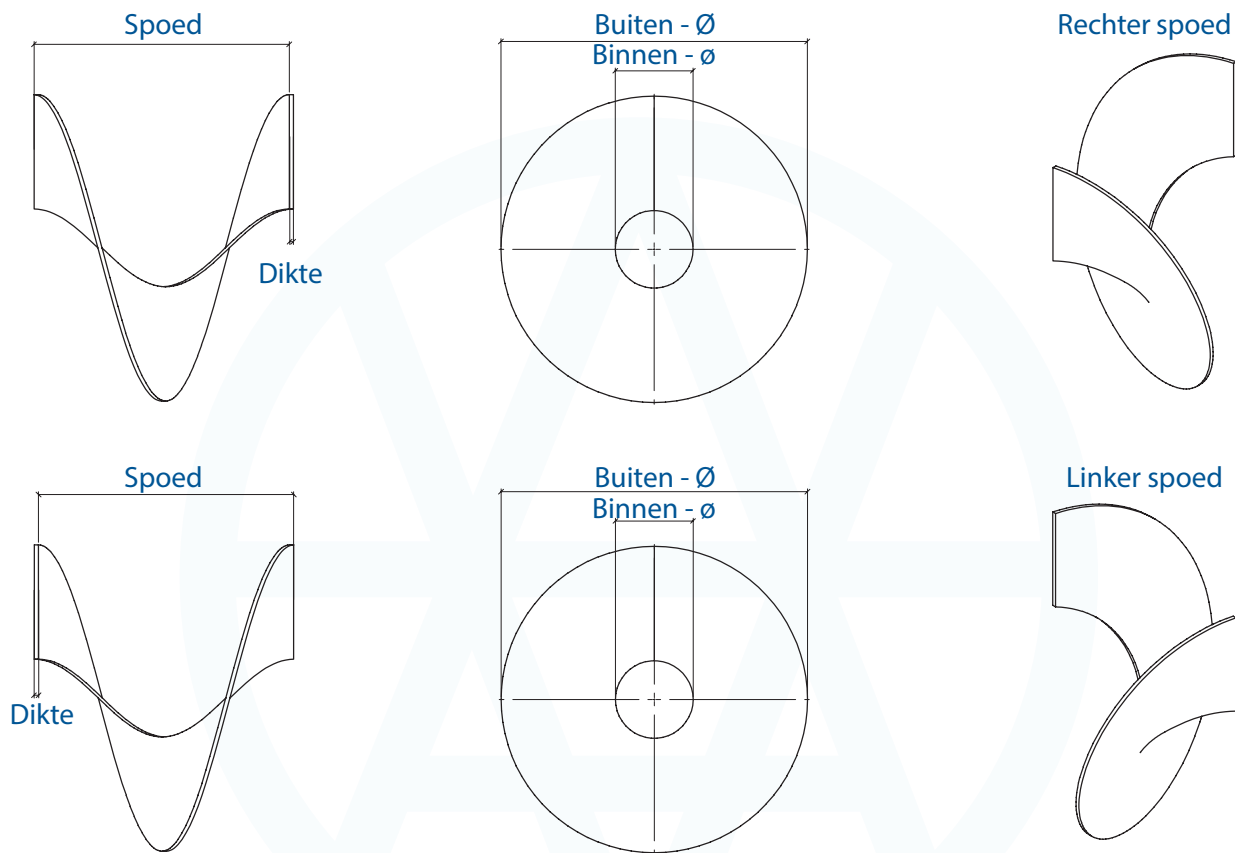
Transportschroefbladen (afmetingen in mm)
