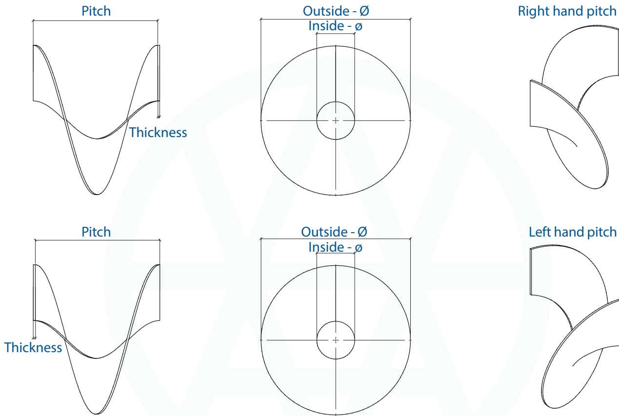
Screw segments (size in mm)
