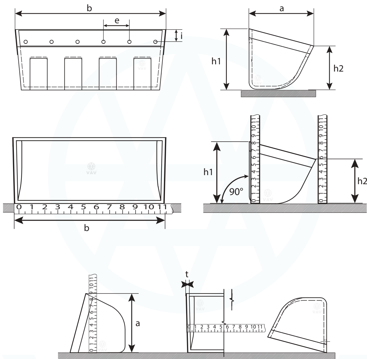
Bucket specifications (sizes in mm)
